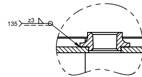
SECTION D-D (SCALE 1:2) WELD SPUD 3/4" NPT - TOP HEAD (4x)
